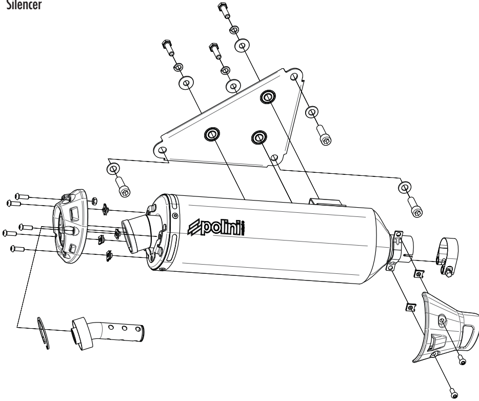
Silencer
